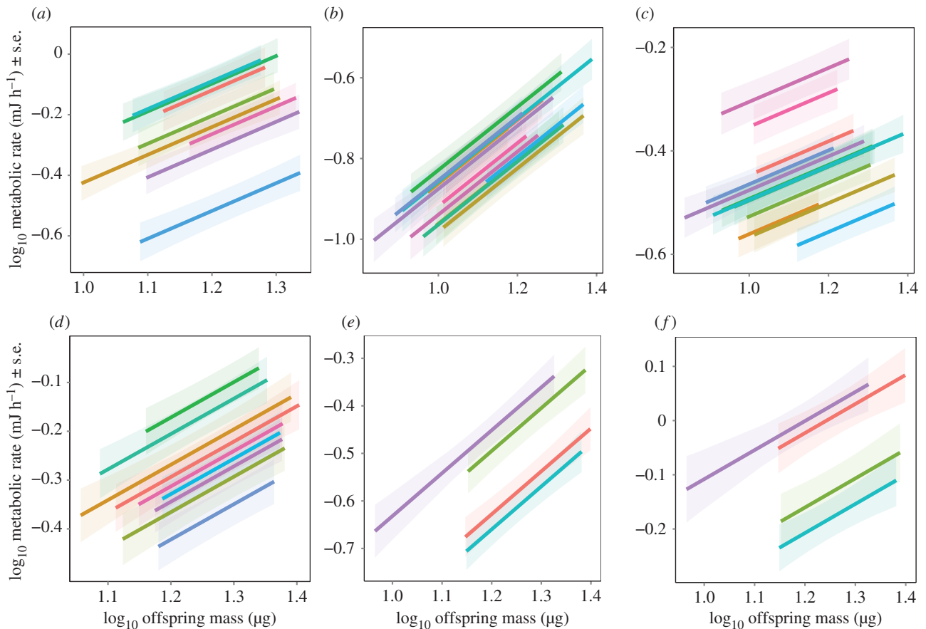
Figure 1. Predicted lines of best fit per experimental run from linear mixed-effects model ( \pm s.e.) for the relationship between \log_{10} offspring mass ( \mu\text{g} ) and \log_{10} metabolic rate ( \text{mJ h}^{-1} ) for B. neritina : (a) larval stage, (b) early post-settlement stage, (c) late post-settlement stage and W. subtorquata : (d) larval stage, (e) early post-settlement stage, (f) late post-settlement stage. Each line represents an experimental run with a common slope and its own unique intercept per development stage.
