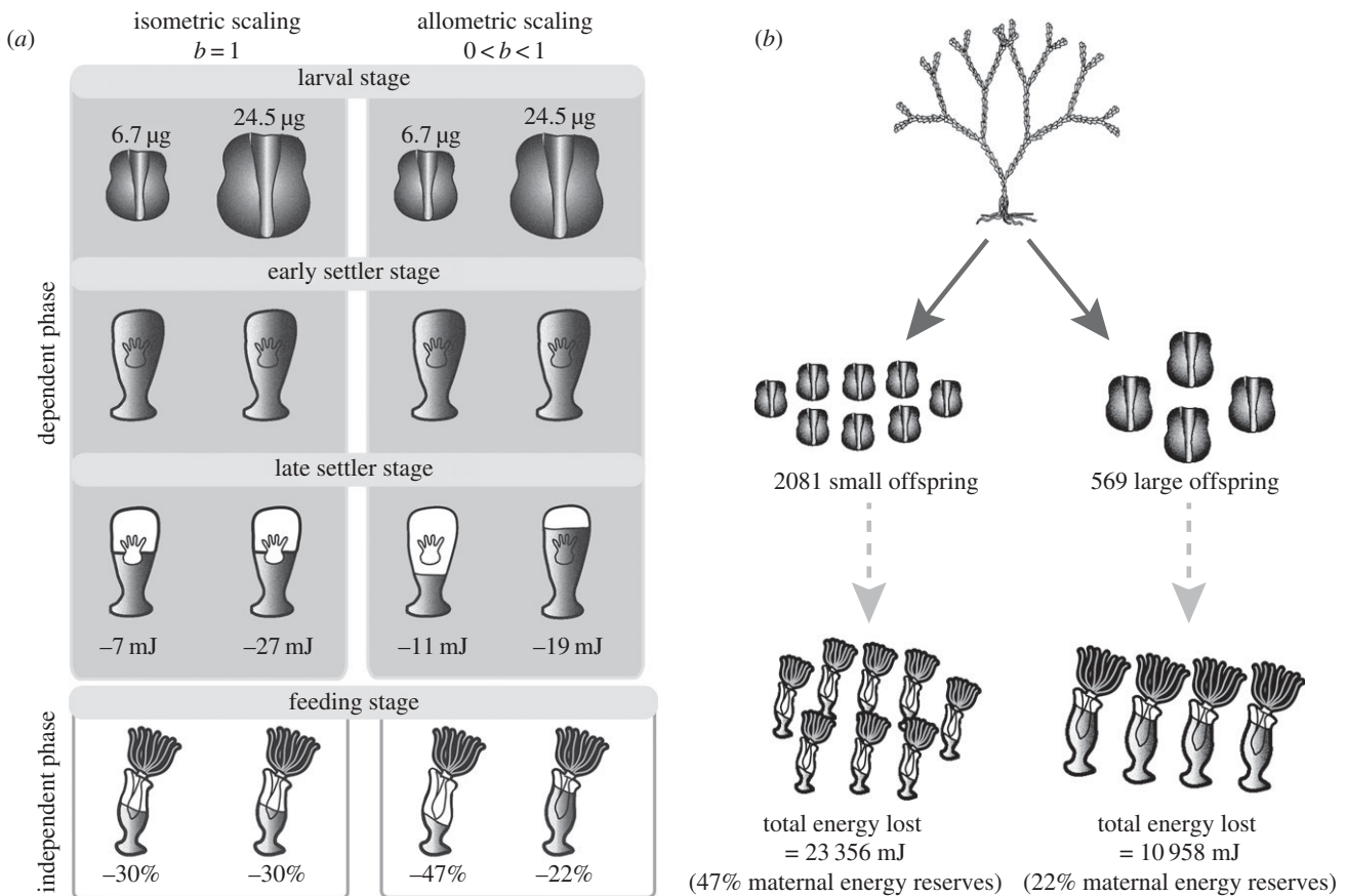
Figure 2. Schematic showing proportion of energy used by the smallest (6.7 \mu\text{g} ) and largest (24.5 \mu\text{g} ) B. neritina larvae observed in our study. (a) Hypothetical isometric relationship (scaling exponent, b = 1 ; as assumed by life-history theory) versus an allometric relationship between size and metabolic rate up until the independent phase based on scaling exponents obtained from our results (larval stage; b = 0.76 , early stage; b = 0.76 , late stage; b = 0.29 ). According to the power function, \text{MR} = aM^b , energy use is directly proportional to body mass in an isometric relationship (where b = 1 ), while in an allometric relationship, smaller offspring use relatively more energy per unit body mass than larger offspring ( b < 1 ). (b) The relative amount of energy that is consumed in the dependent phase for mothers with identical total reproductive investments (fecundities based on field observations at our field site) but where one mother produces the largest observed offspring and the other produces the smallest observed offspring. As a proportion of total supplied energy, the fewer, larger offspring in total will use less than half of the maternally supplied energy relative to the many smaller offspring (i.e. mother producing larger offspring: total energy (50 000 mJ)/per offspring energy (87.9 mJ) = offspring number (569) \times individual energy burned (19.3) = total metabolic cost (10 958 mJ)).
